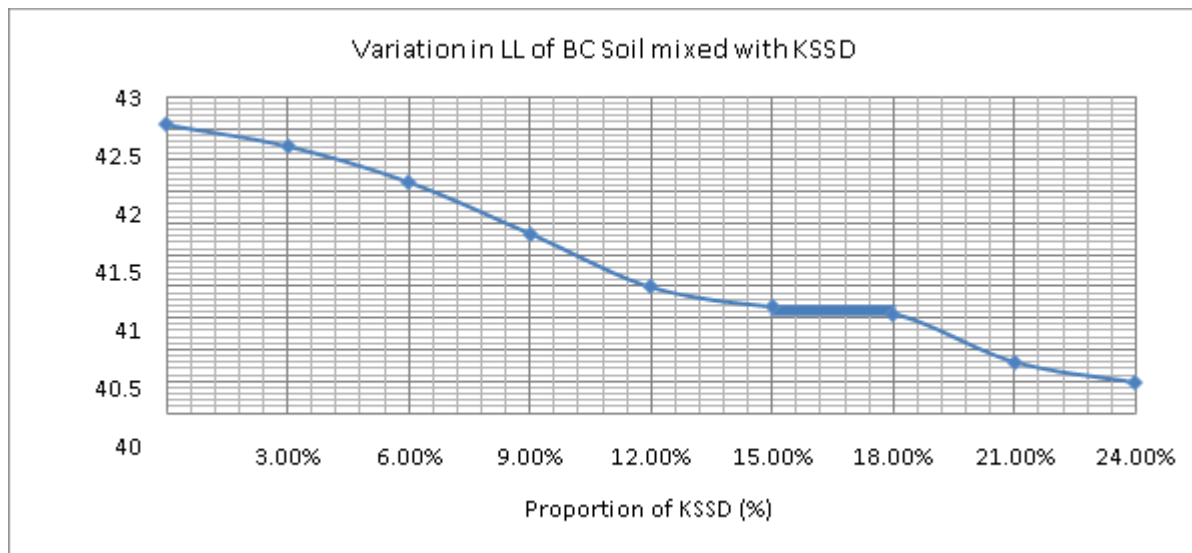
Fig 3: Variation in Liquid Limit value for the BC Soil mixed with Kota stone slurry dust
