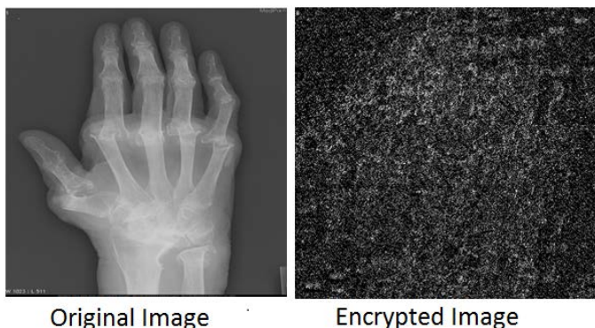
Figure 1 : Image Encryption
