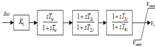
Fig 2: Structure of PSS [10]
