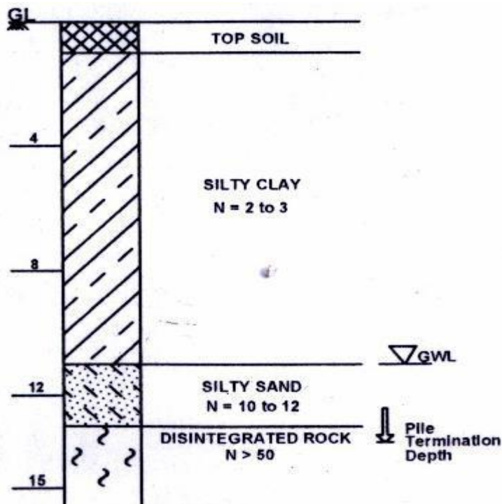
Figure 1 : Soil Profile Bailer System Piling
