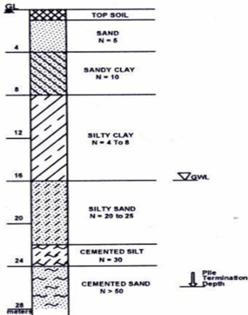
Figure 7 : Soil Profile Rotary Piling
