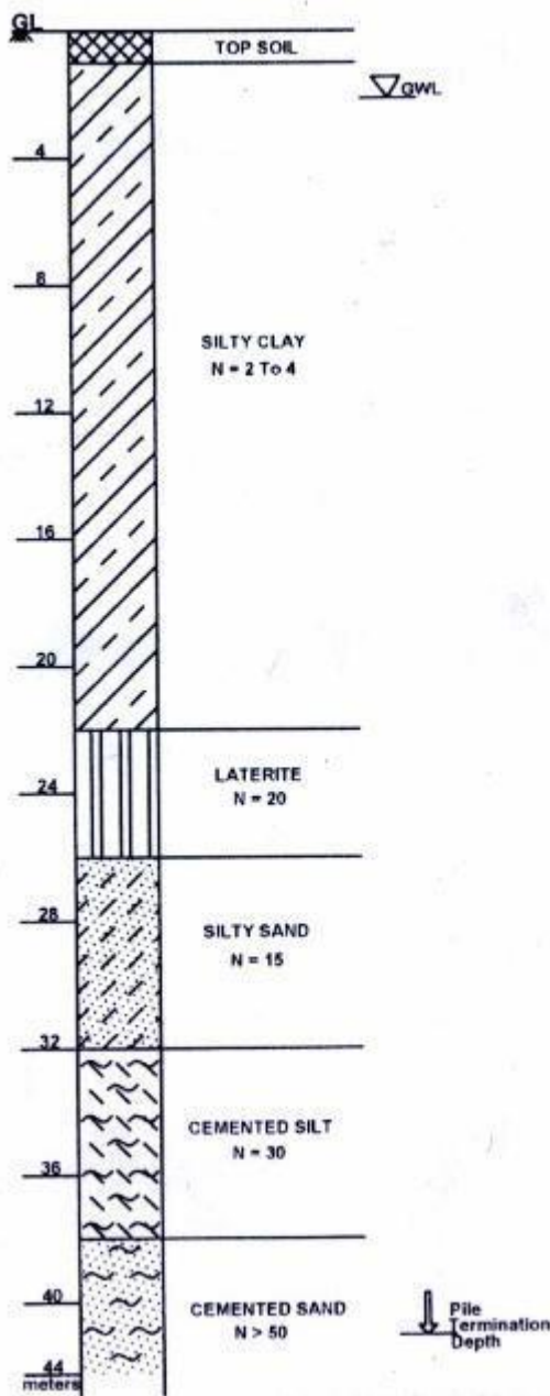
Figure 3 : Soil Profile DMC Piling
