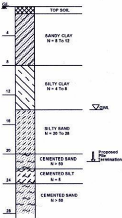
Figure 5 : Soil Profile Driven Piling
