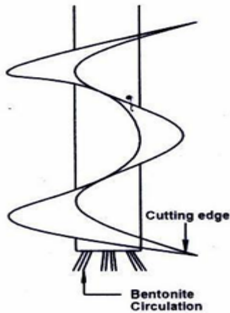
Figure 8 : Rotary Auger System
