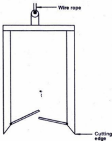
Figure 2: Bailer with Flap Door
