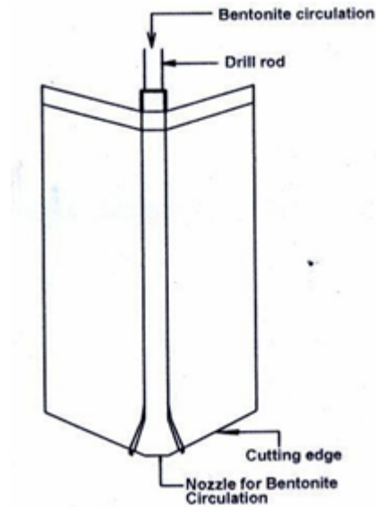
Figure 4: DMC Chisel
