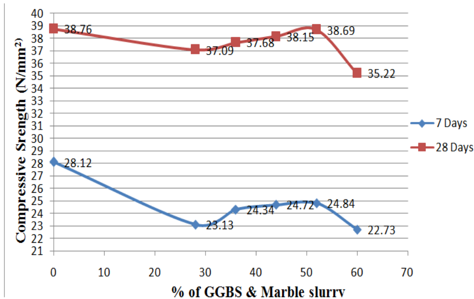
Fig. 5: Effect of Ground- granulated blast furnace slag and Marble slurry on concrete of M25 grade on replacement for 7 and 28 days compressive strength of cube
