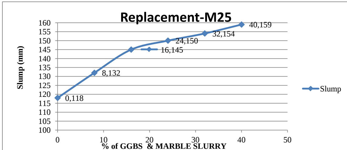
Fig. 4: Effect on Replacement of OPC by Ground-granulated blast-furnace slag and fine aggregate by Marble slurry For M25 Grade
