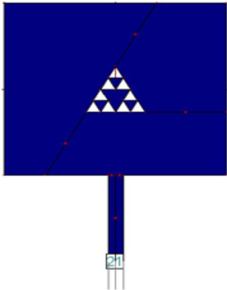
Fig. 3: Geometry of first iteration of proposed fractal antenna
