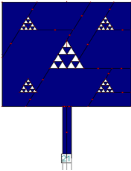
Fig.7: Geometry of second iteration of proposed fractal antenna
