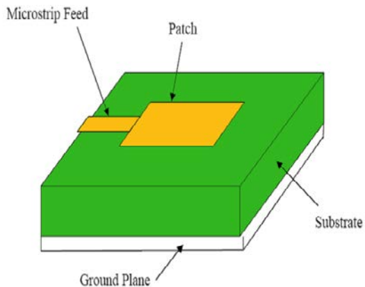
Fig. 2: Microstrip Line Feed
