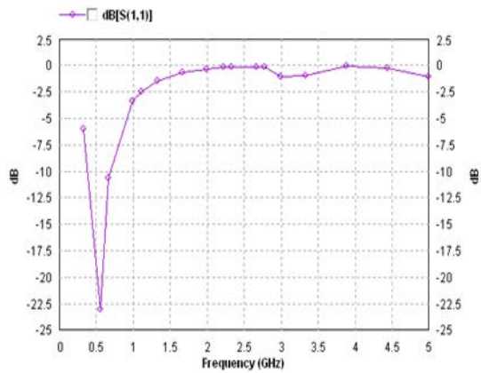
Fig. 4: Return loss versus frequency plot of 1 st iteration of proposed fractal antenna
