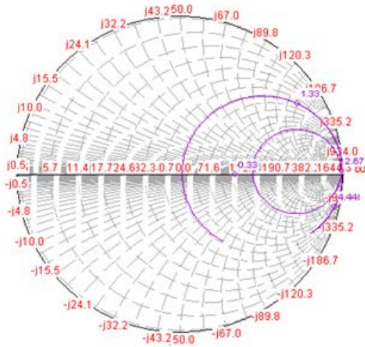
Fig.10: Input impedance loci using smith chart of 2 nd iteration of proposed fractal antenna
