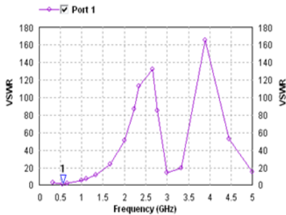
Fig.13: VSWR versus frequency plot of 3 rd iteration of proposed fractal antenna
