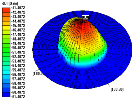
Fig.15: Gain of 3 rd iteration of proposed fractal antenna
