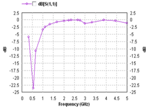
Fig.12: Return loss vs. frequency plot of 3 rd iteration of proposed fractal antenna
