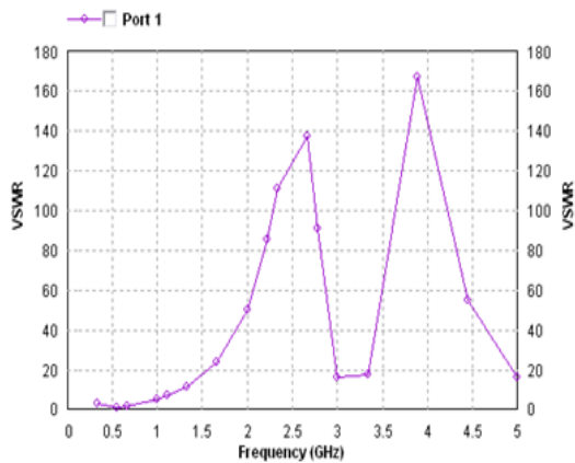
Fig. 5: VSWR versus frequency plot of I st iteration of proposed fractal antenna
