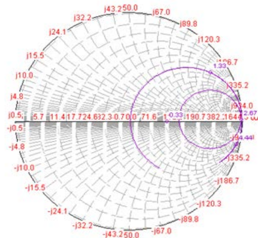
Fig.14: Input impedance loci using smith chart of 3 rd iteration of proposed fractal antenna
