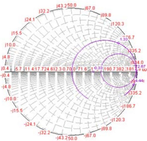
Fig.6: Input impedance loci using smith chart of 1 st iteration of proposed fractal antenna
