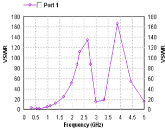
Fig.9: VSWR versus frequency plot of 2 nd iteration of proposed fractal antenna
