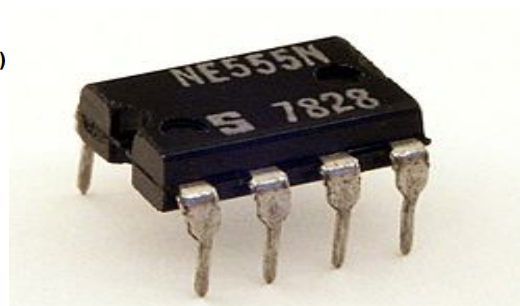
Figure 5: 555 Timer with PIN diagram
