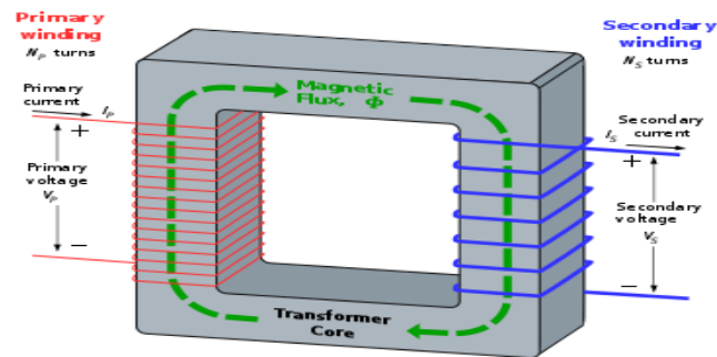
Figure 3: Transformer with Flux Linkages
