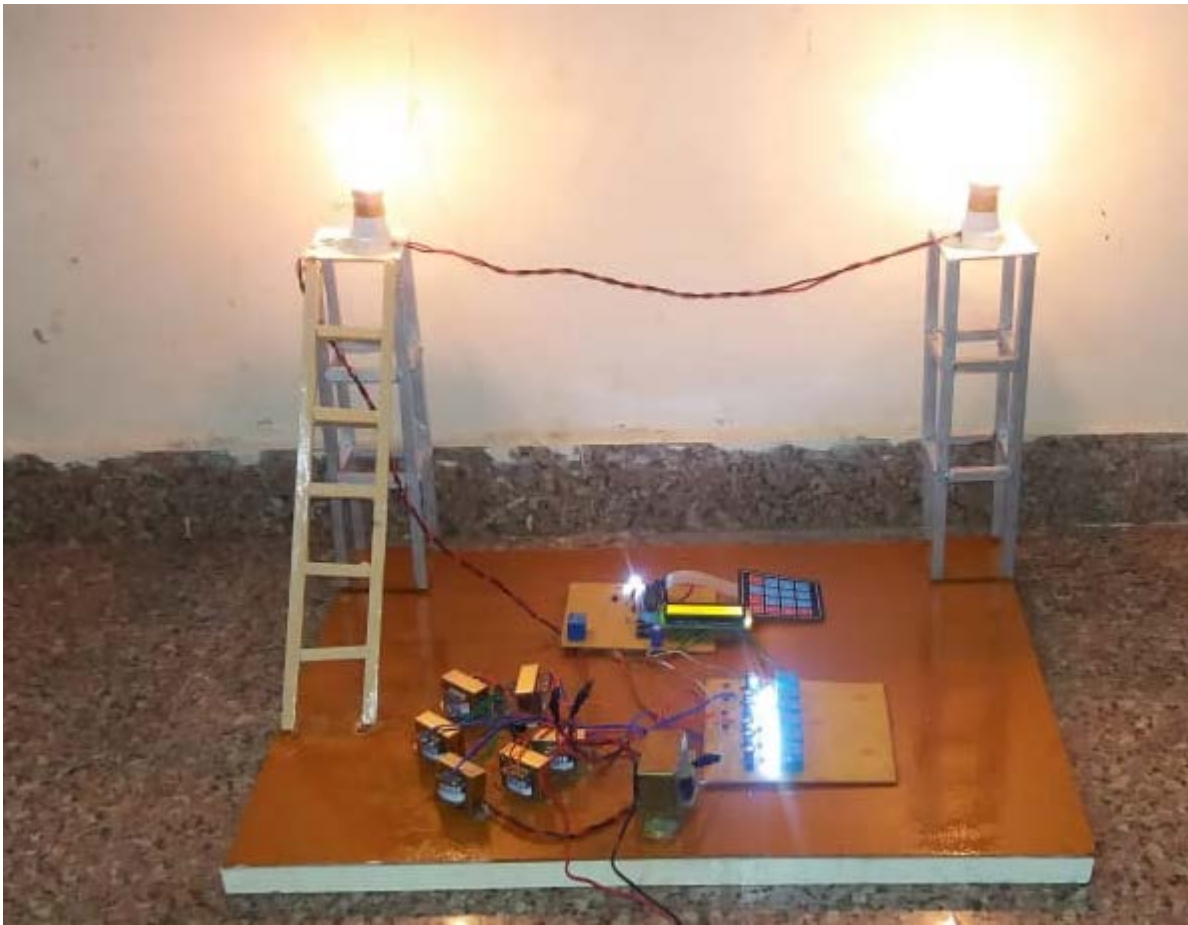
Figure 2: Image of Hardware
