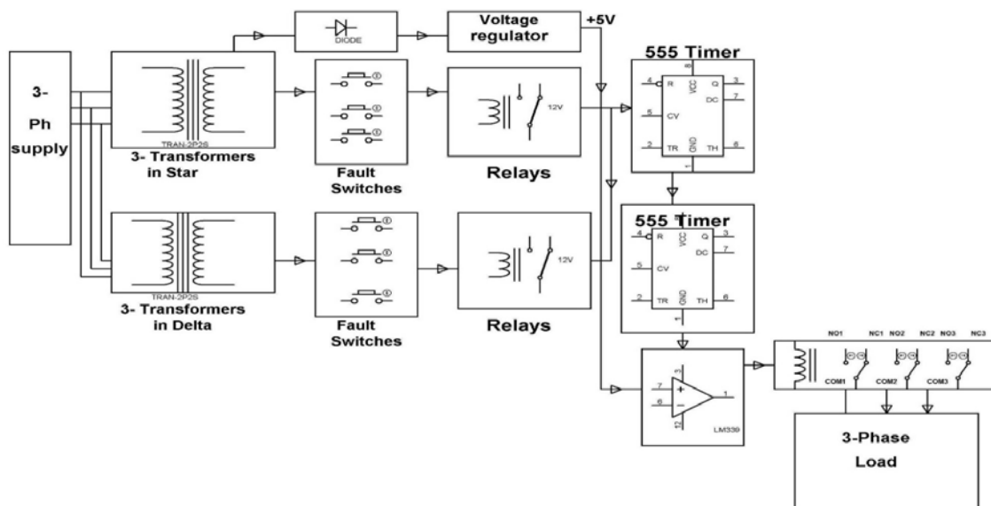
Figure 1: Block Diagram of Three Phase Fault Analysis
