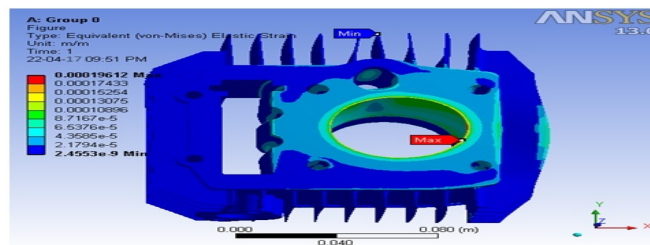
Figure 5.9: Variation of Strain for Group 0 (Pure Alloy)
