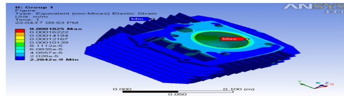
Figure 5.11: Variation of Strain for Group 1
