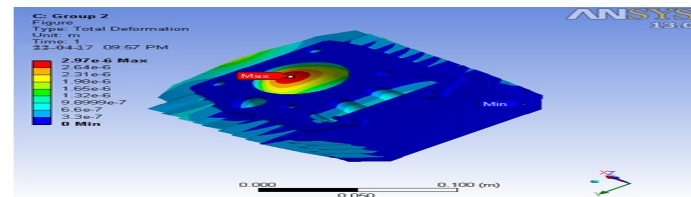
Figure 5.12: Variation of Total Deformation for Group 2
