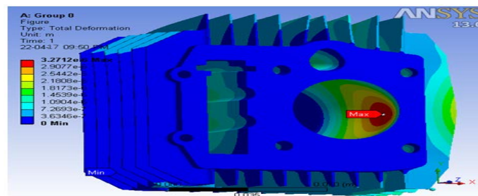
Figure 5.8: Variation of Total Deformation for Group 0 (Pure Alloy)
