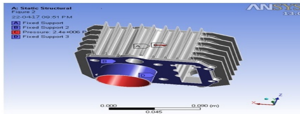
Figure 5.6: Boundary Conditions and Constraints Defined to Model
