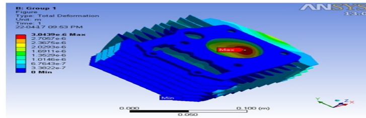
Figure 5.10: Variation of Total Deformation for Group 1
