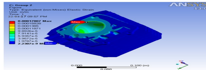
Figure 5.13: Variation of Strain for Group 2
