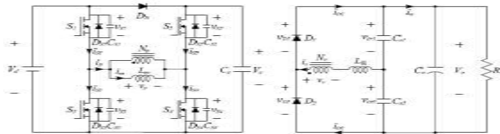
Figure 1: Circuit diagram of the proposed hybrid-type full bridge dc/dc converter
