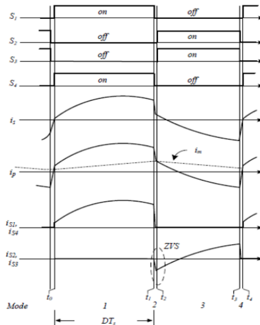
Figure 5: Operation waveforms in the active-clamp step-up converter mode
