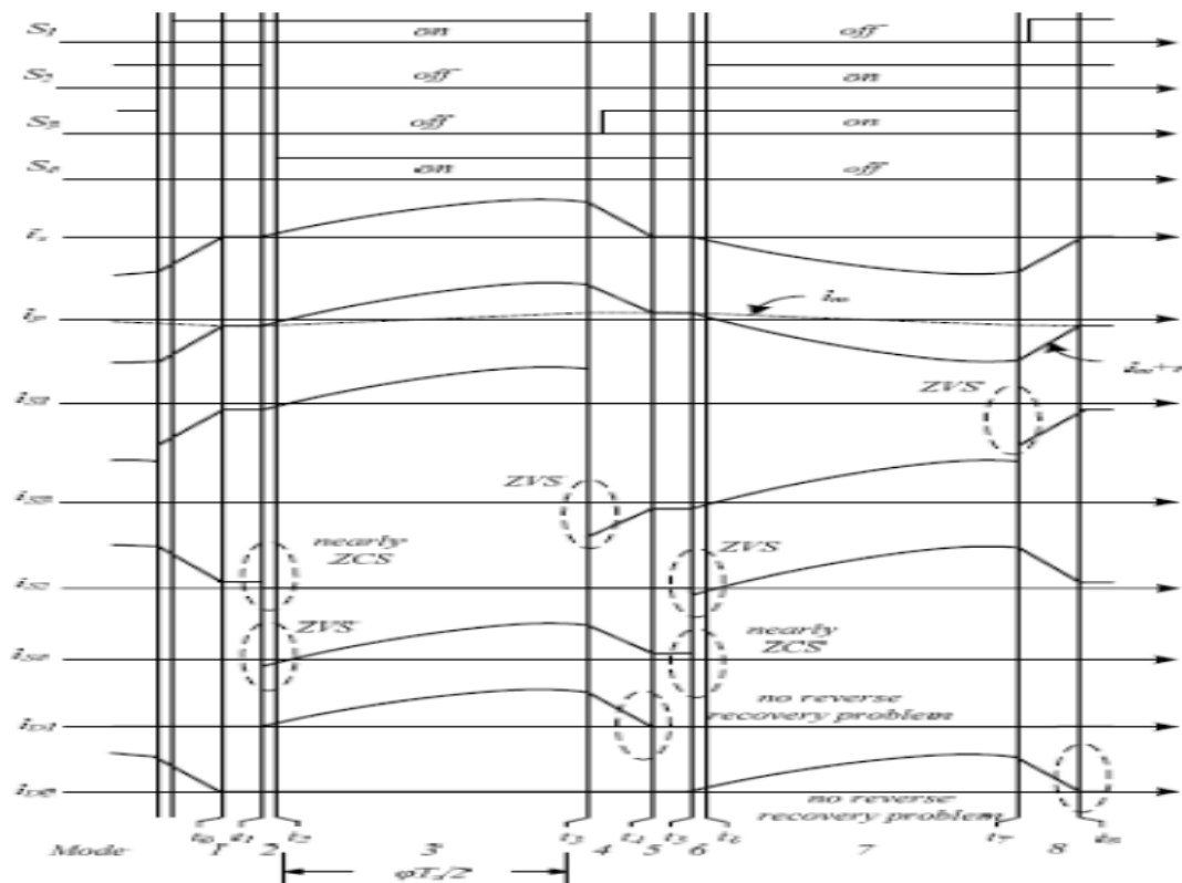
Figure 3: Operation waveforms in the PSFB series resonant converter mode.
