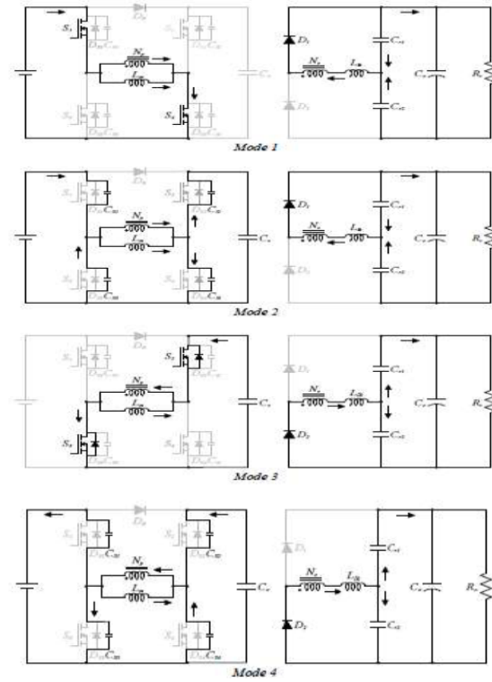
Figure 4: Equivalent circuits during a switching period in the active-clamp step-up converter mode.
