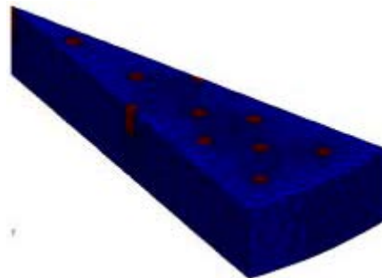
Figure 4: Discretisation of the 3D model of the sample with water trees
