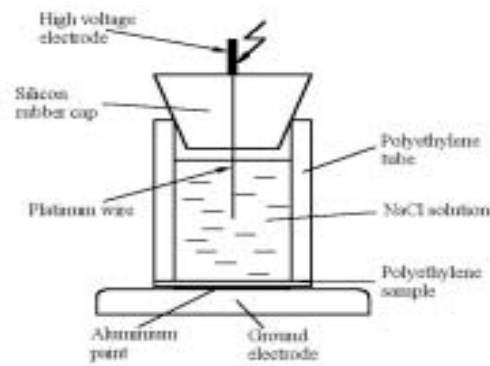
Figure 1: Cell used to produce water trees
